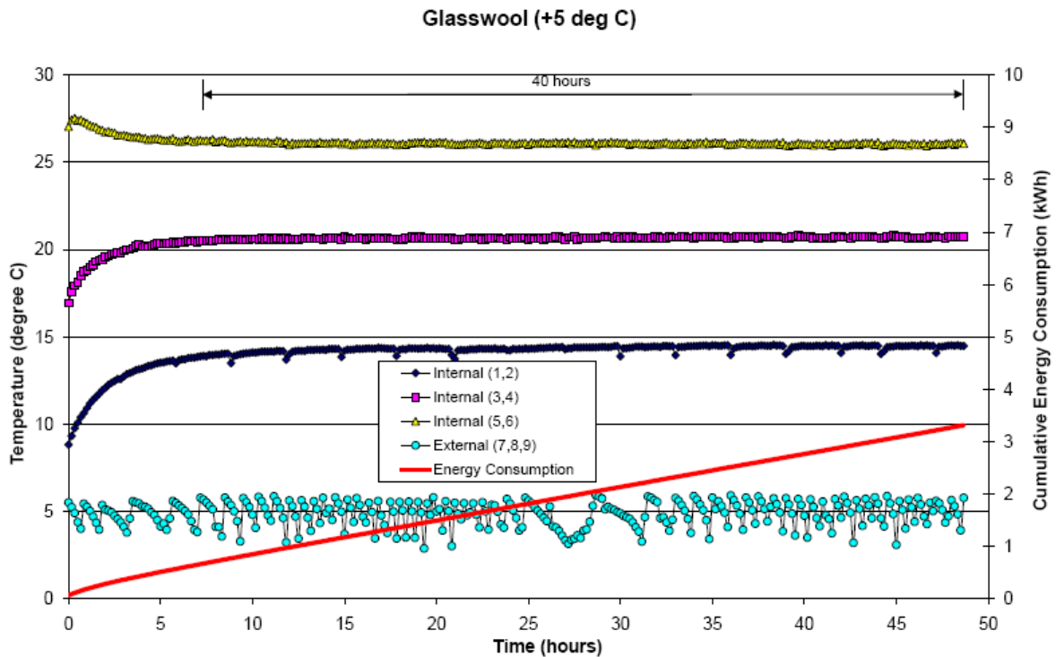
Fig. 13 Temperature profiles at +5°C
